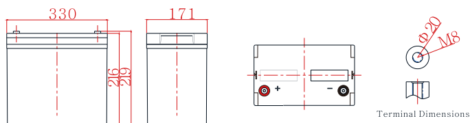
Terminal Dimensions
